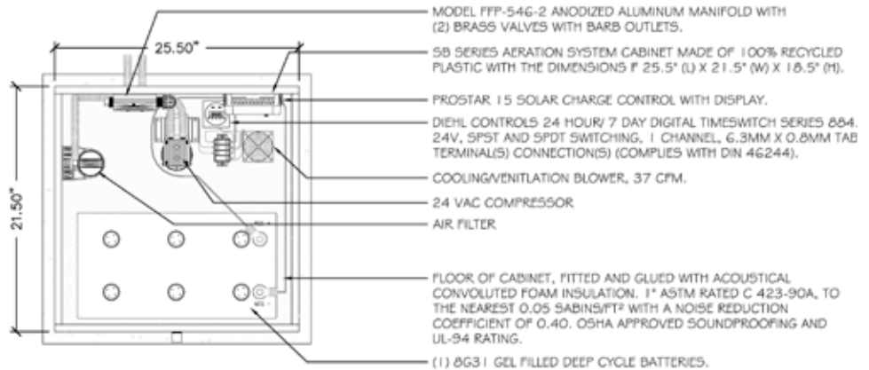
TOP VIEW NOT TO SCALE
