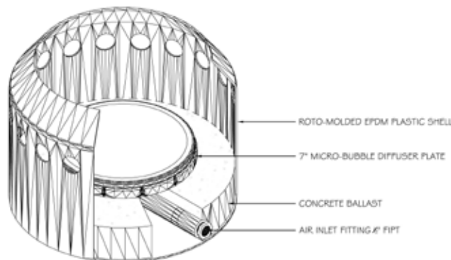
DURAPLATE DIFFUSER DDP-7 - CUT VIEW NOT TO SCALE
